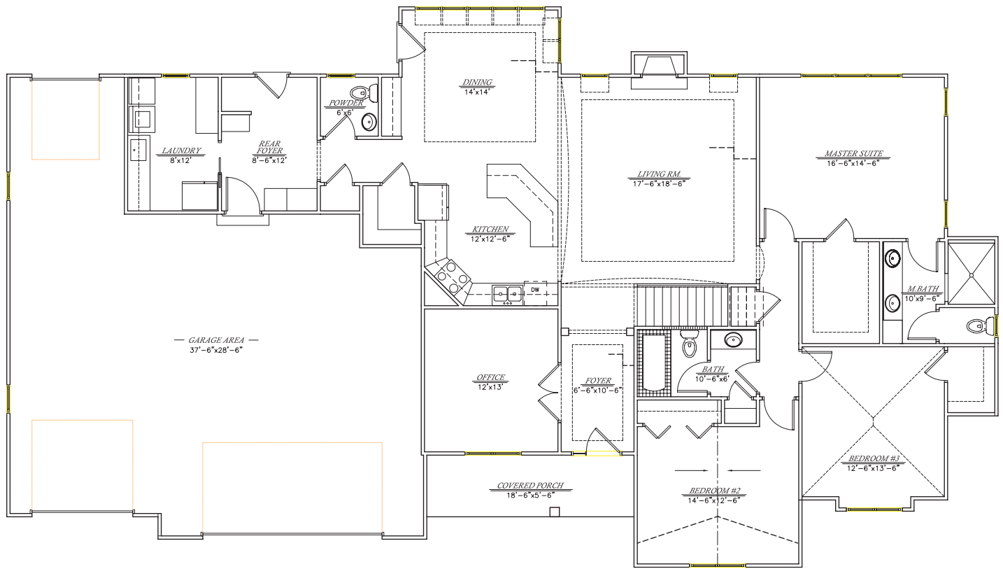
CHARLESTON I 2290 SQ. FT.
